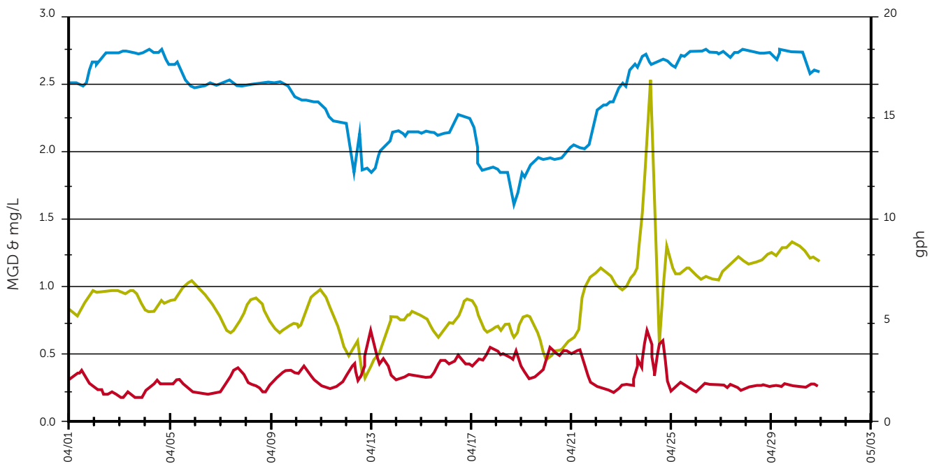
Figure 2: RTC-P is in control: By getting real-time test data every 5-7 minutes, 288 times per day, the plant is able to detect phosphorus changes quickly, monitor quality, dose as needed and adjust set-points throughout the week. The plant is successfully keeping TP levels well under the average discharge limit.
